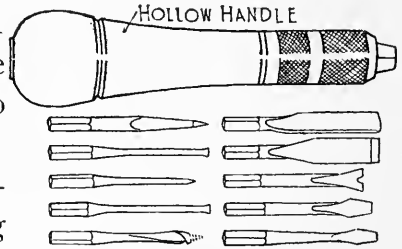
FIG. 91. PATENT AWL.
